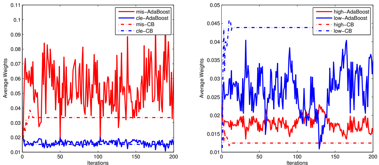
Fig. 2. Average weights of different types of instances during the learning process in the original AdaBoost and CB-AdaBoost. The left panel is for weights of mislabelled instances and clean-labelled instances. The right panel is for weights of groups with high and low label confidence.
