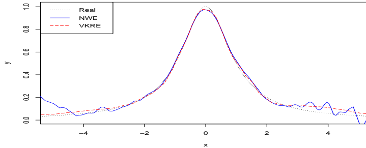
Figure 2: y = 1/(x^2 + 1)
