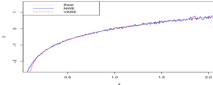
Figure 3: y = \log|x|
