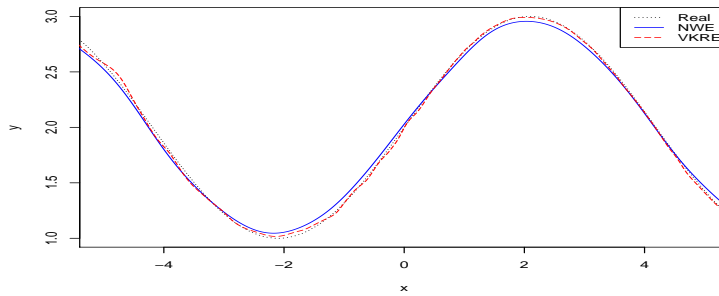
Figure 1: y = 2 + \sin(0.75x)
